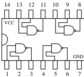
74LS03
